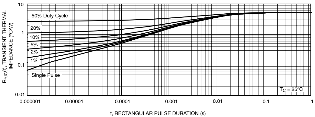
Figure 14. Thermal Response
