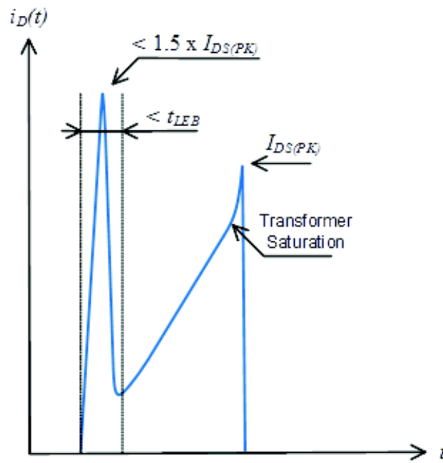
Figure 3. Spike Limits
