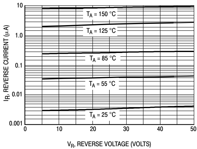
Figure 3. Leakage Current
