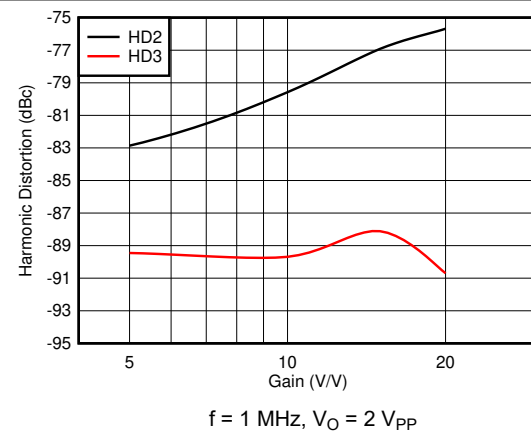
Figure 5-18. Harmonic Distortion vs Gain
