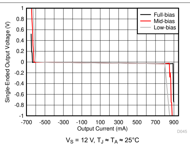
Figure 6-2. Linear Single-Ended Output Voltage vs I_O and Temperature
