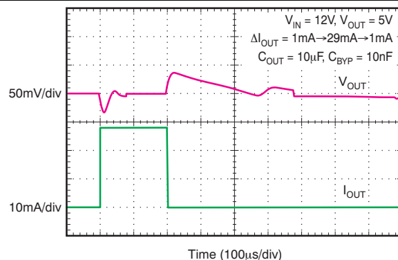
Figure 2. Load Transient Response
