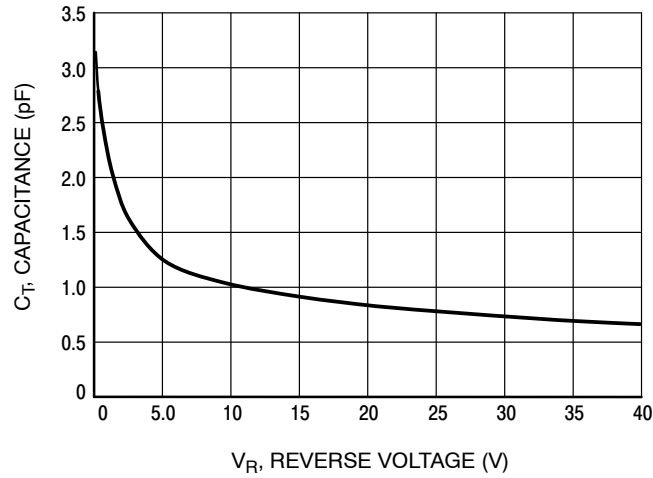
Figure 4. Typical Capacitance
