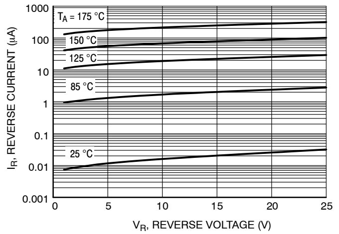
Figure 3. Reverse Current versus Reverse Voltage
