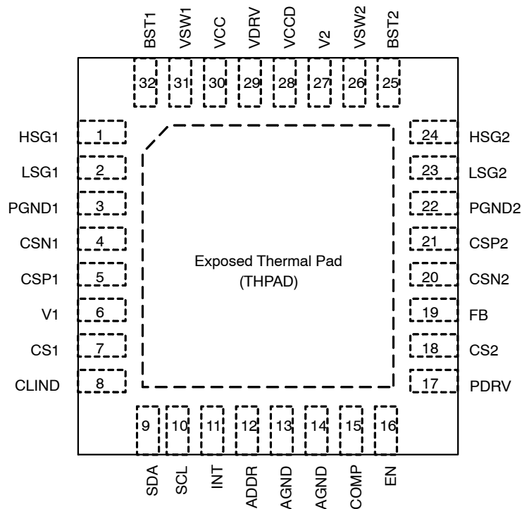
Figure 2. Pinout
