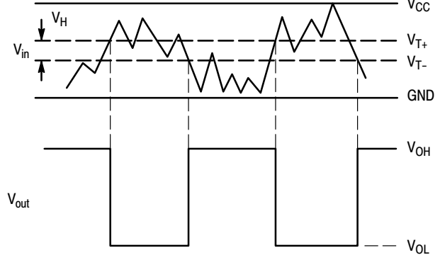
Figure 6. Typical Schmitt-Trigger Applications
