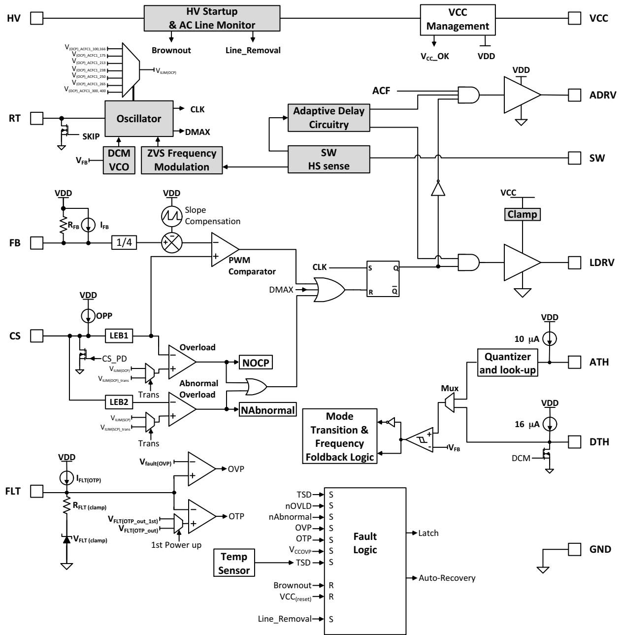
Figure 3. Block Diagram
