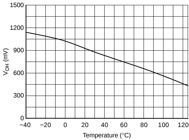
Figure 20. High-Level Output Voltage vs. Temperature
