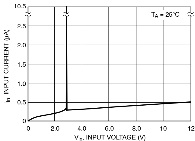
Figure 4. NCP300/1 Series 2.7 V Input Current versus Input Voltage
