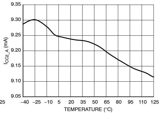
Figure 36. Internal IC Consumption (A Version, C_{DRV} = 1 \text{ nF} , f_{SW} = 400 \text{ kHz} , t_{on\_min} = 500 \text{ ns} , t_{off\_min} = 620 \text{ ns} )
