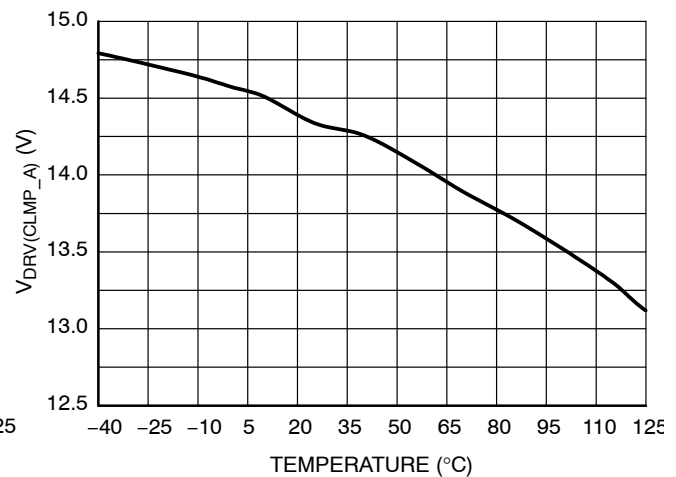
Figure 16. Driver Clamp Level – A Version, V_{CC} = 28\text{ V} and C_{DRV} = 10\text{ nF}
