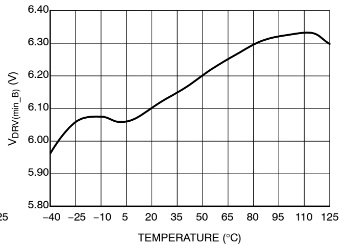
Figure 14. Minimal Driver High Level – B Version, V_{CC\_off} + 0.2\text{ V} and C_{DRV} = 0\text{ nF}
