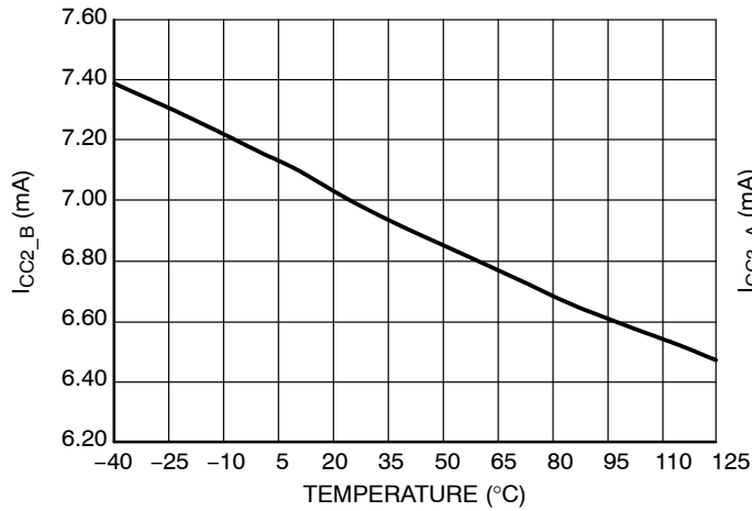
Figure 37. Internal IC Consumption (B Version, C_{DRV} = 1 \text{ nF} , f_{SW} = 400 \text{ kHz} , t_{on\_min} = 500 \text{ ns} , t_{off\_min} = 620 \text{ ns} )
