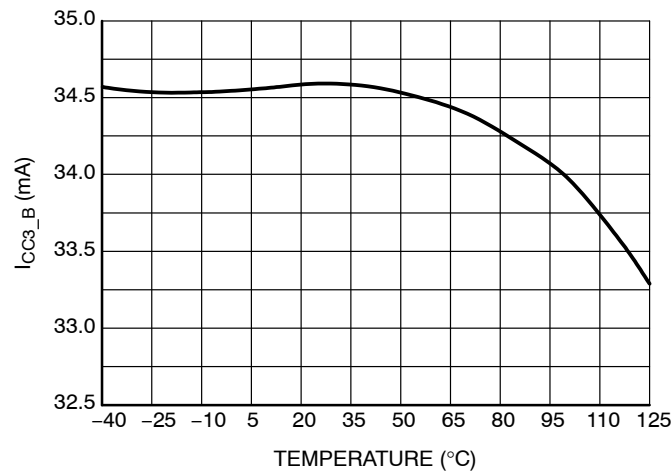
Figure 39. Internal IC Consumption (B Version, C_{DRV} = 10 \text{ nF} , f_{SW} = 400 \text{ kHz} , t_{on\_min} = 500 \text{ ns} , t_{off\_min} = 620 \text{ ns} )
