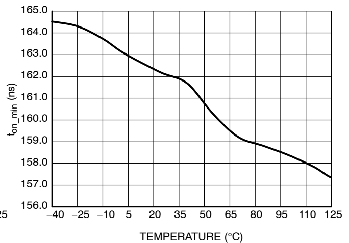
Figure 28. Minimum on Time @ R_{MIN\_TON} = 0 \Omega
