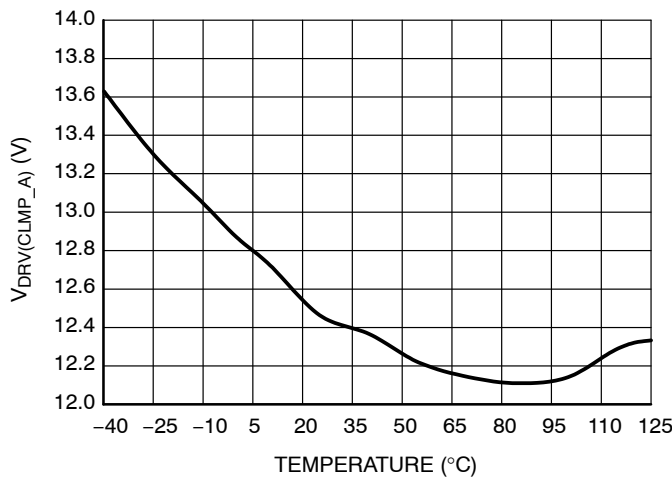
Figure 15. Driver Clamp Level – A Version, V_{CC} = 28\text{ V} and C_{DRV} = 1\text{ nF}
