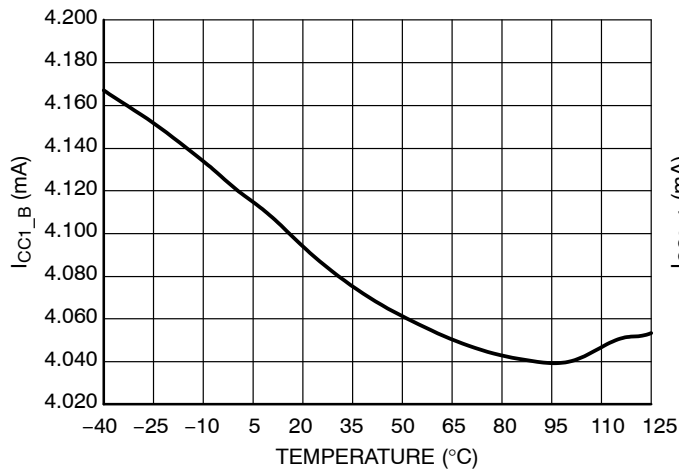
Figure 35. Internal IC Consumption (B version, C_{DRV} = 0 \text{ nF} , f_{SW} = 500 \text{ kHz} , t_{on\_min} = 500 \text{ ns} , t_{off\_min} = 620 \text{ ns} )
