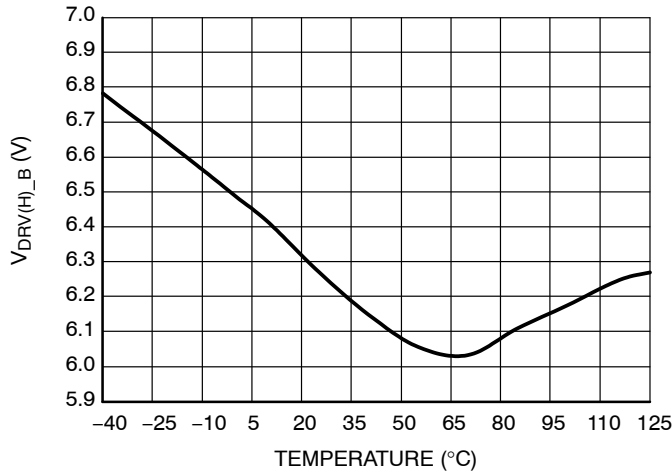
Figure 11. Driver High Level – B Version, V_{CC} = 12\text{ V} and C_{DRV} = 1\text{ nF}
