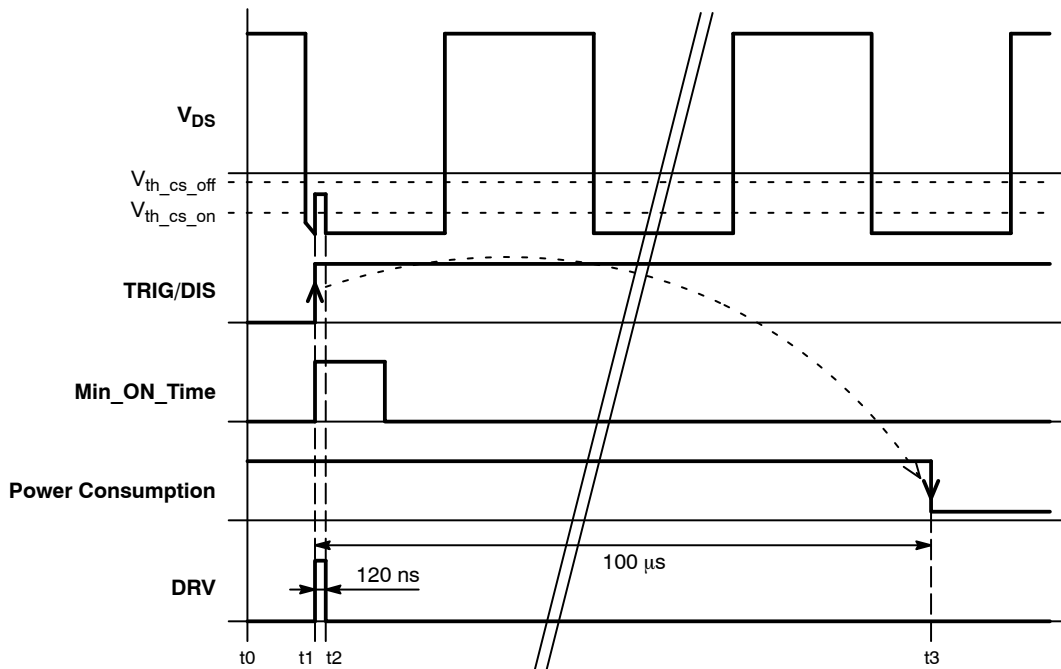
Figure 55. TRIG/DIS from LOW to HIGH Sequence 2
