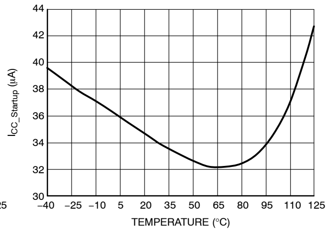
Figure 8. Startup Current
