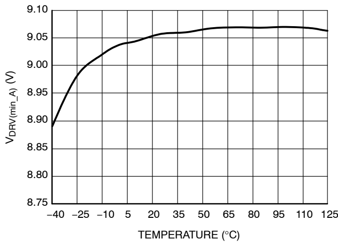
Figure 13. Minimal Driver High Level – A Version, V_{CC\_off} + 0.2\text{ V} and C_{DRV} = 0\text{ nF}
