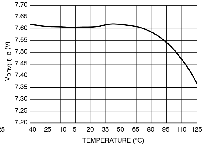
Figure 12. Driver High Level – B Version, V_{CC} = 12\text{ V} and C_{DRV} = 10\text{ nF}
