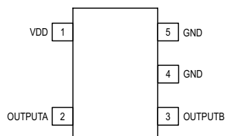
Package LH, 5-Pin SOT23W Pinout
