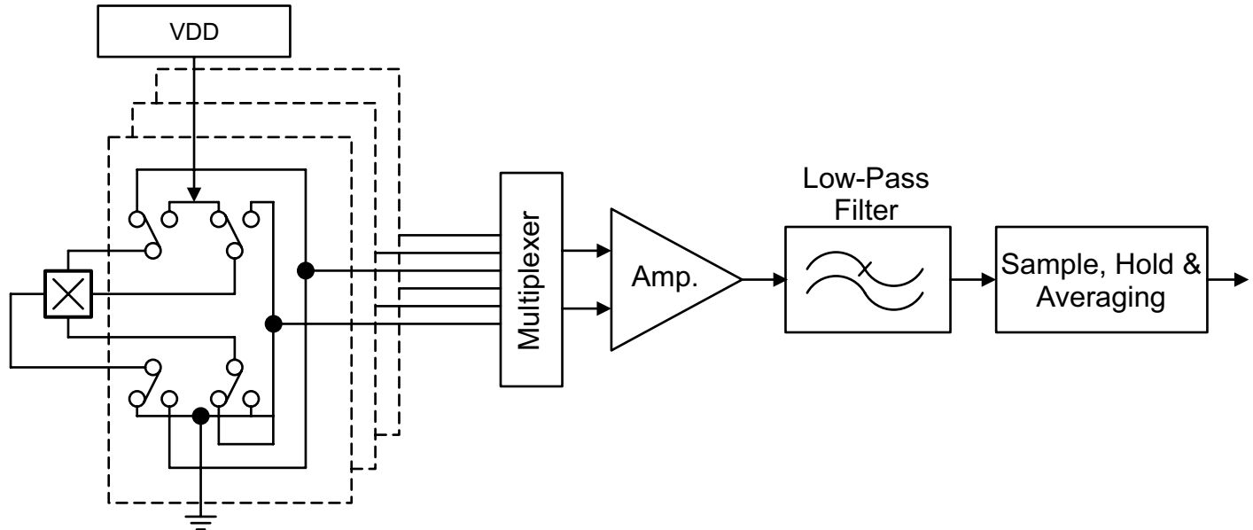
Figure 11: Model of Chopper Stabilization Technique
