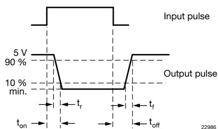
Fig. 11 - Switching Waveform
