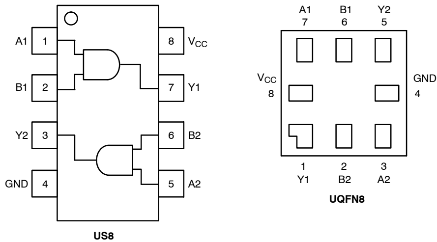
Figure 2. Pinout
