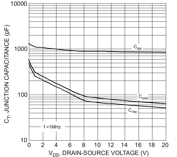
Figure 20 Typical Junction Capacitance
