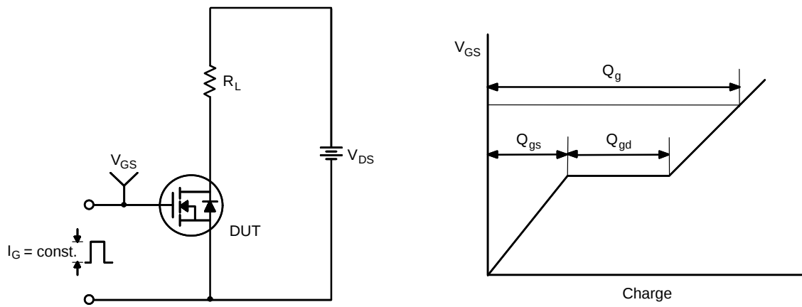
Figure 13. Gate Charge Test Circuit &amp; Waveform
