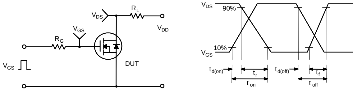
Figure 14. Resistive Switching Test Circuit &amp; Waveforms
