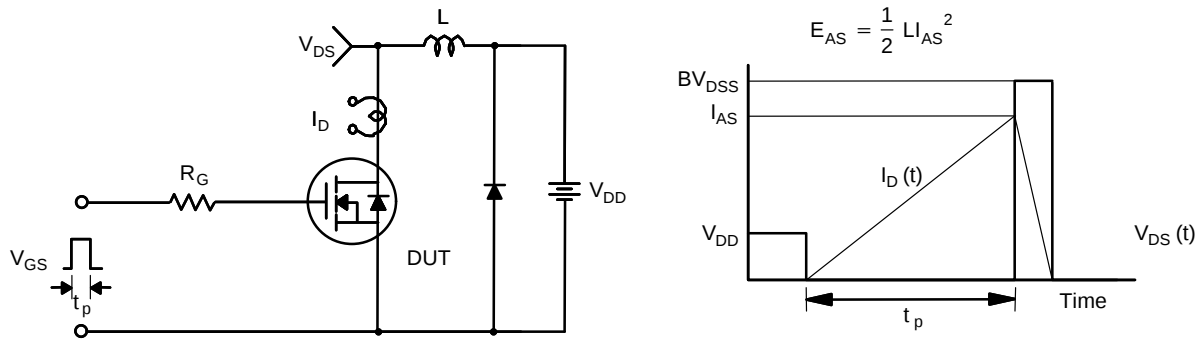
Figure 15. Unclamped Inductive Switching Test Circuit &amp; Waveforms
