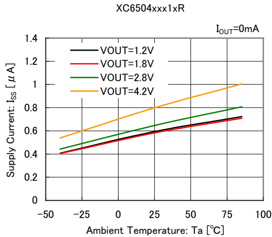
(7) Supply Current vs. Ambient Temperature
