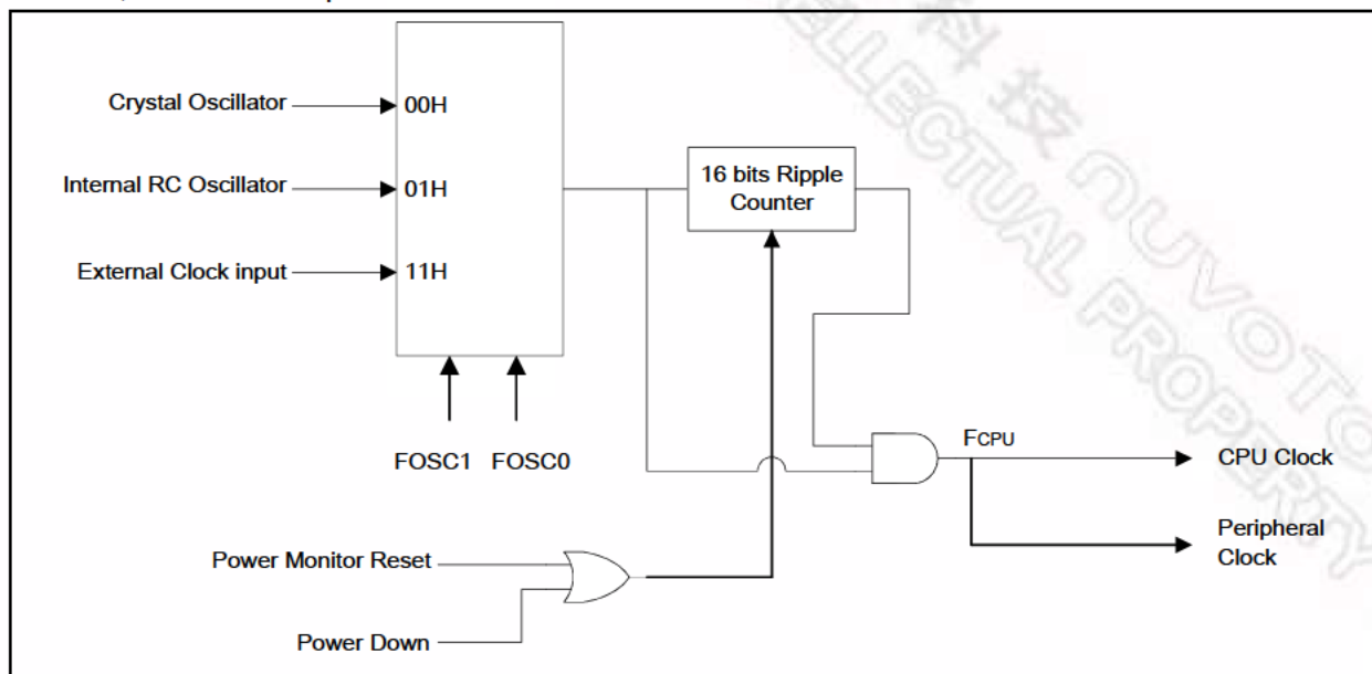
Figure 21-1: Oscillator
