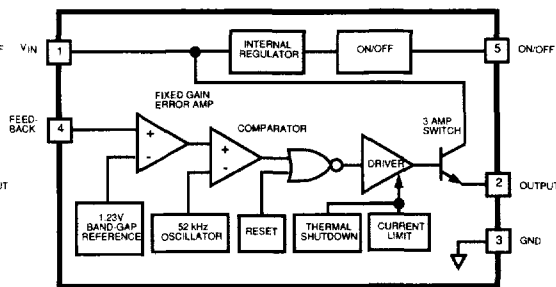
Adjustable Regulator
