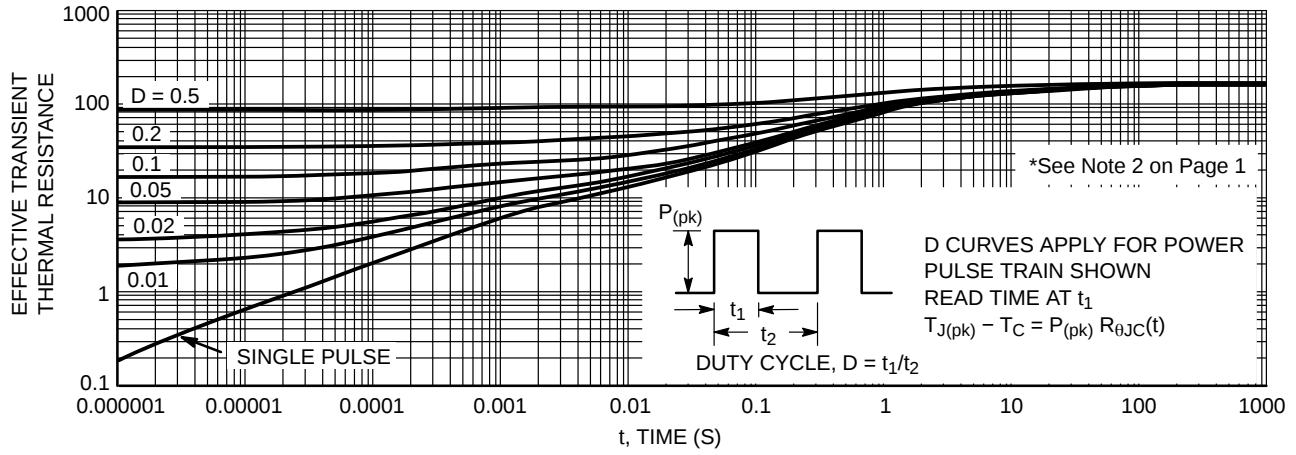
Figure 12. Thermal Response
