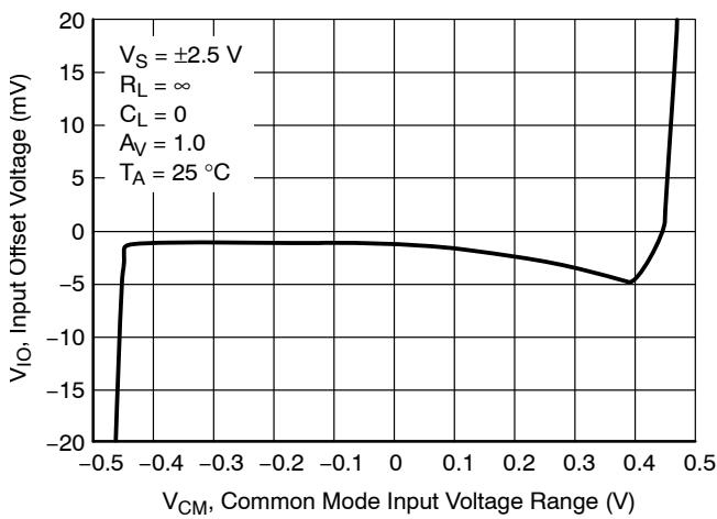
Figure 28. Input Offset Voltage vs. Common Mode Input Voltage Range, V_S = \pm 0.45\text{ V}
