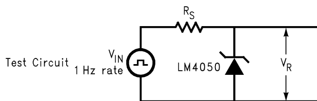
Figure 6-1. Test Circuit
