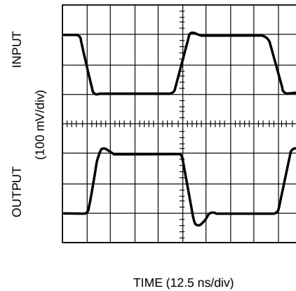
Figure 21. Inverting Small Signal Pulse Response ( V_S = 5\text{V} )
