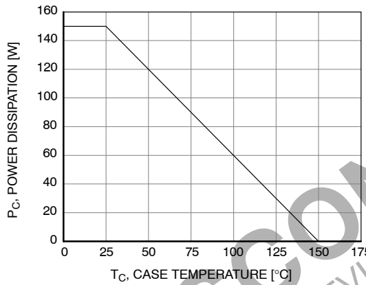
Figure 9. Power Derating
