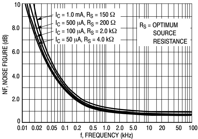
Figure 9. Frequency Effects
