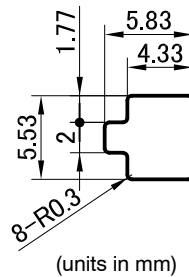
Figure 47. Dimensions of the Protective Foil
