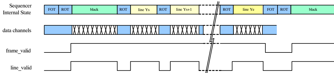
Figure 38. CMOS Mode: Frame Timing Indication
