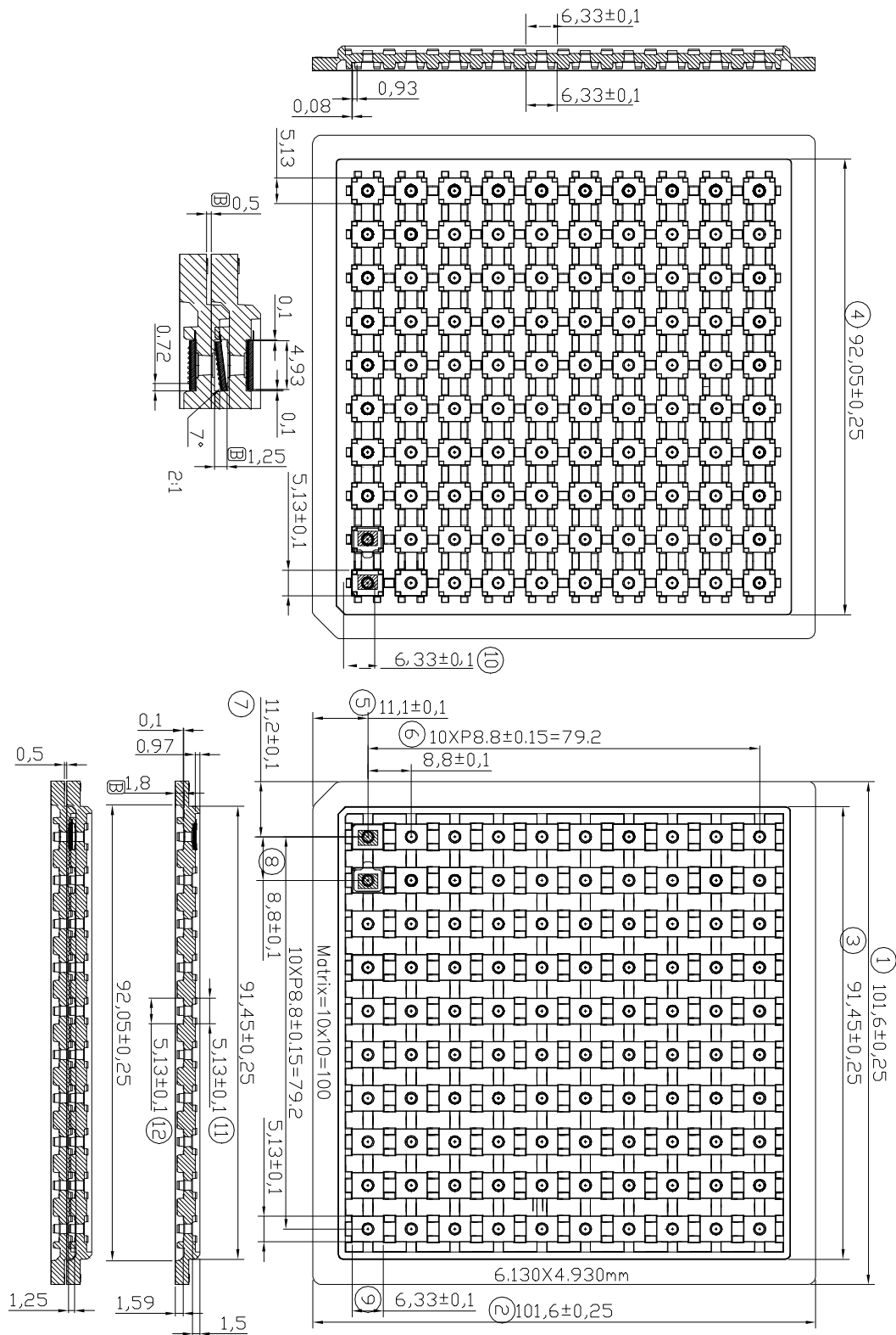
Figure 44. Tray Drawing
