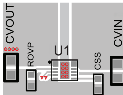
Figure 24. Top Layer Layout. Maximum Number of VIAs from Top Layer Exposed Pad to Inner Layer.
