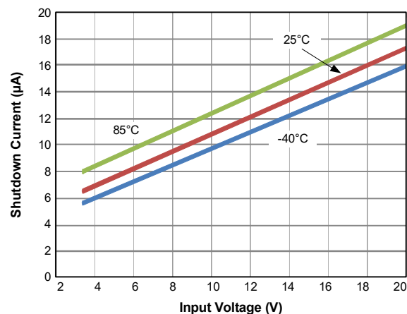
Figure 16. Shutdown Current vs. Input Voltage
