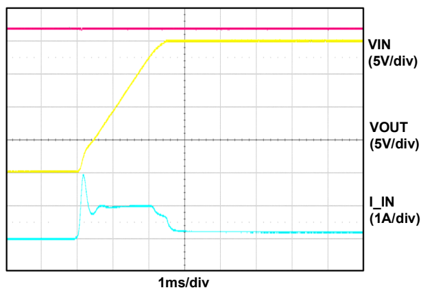
Figure 6. Soft Start Ramp (VIN = 20V)
