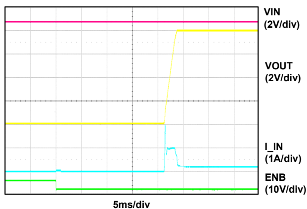
Figure 4. Soft Start Delay Times (VIN = 20V)
