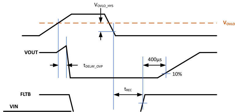
Figure 2. OVP Delay and Recovery Time (AOZ1327DI-01)
