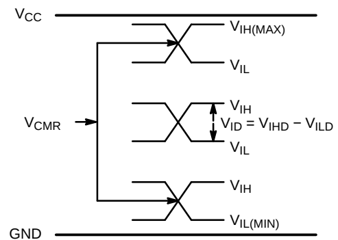
Figure 8. V_{CMR} Diagram
