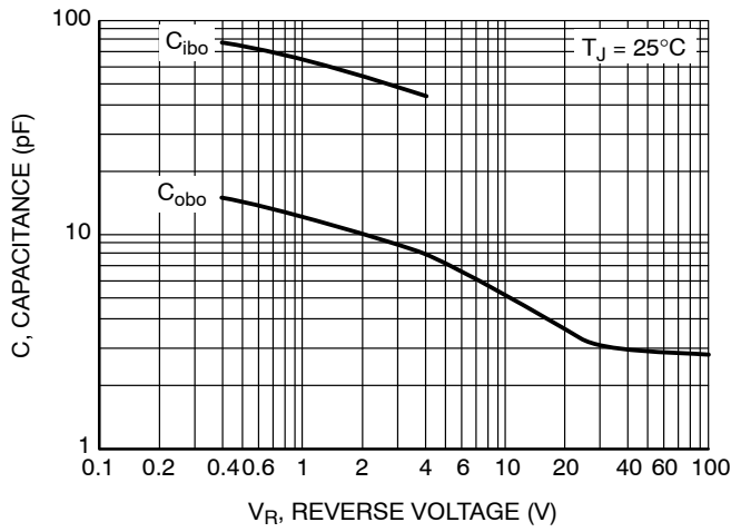
Figure 7. Capacitance
