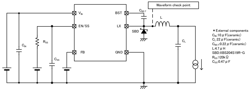
<Circuit No.⑥>
