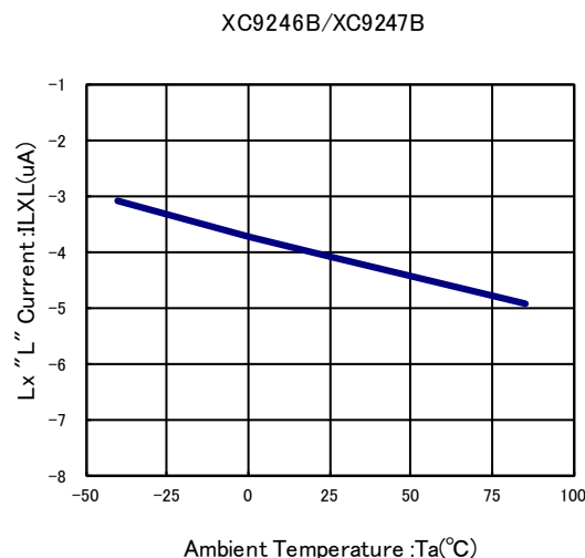
(11) Lx "L" Current vs. Ambient Temperature
