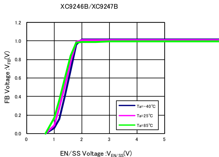
(13) FB Voltage vs. EN/SS Voltage
