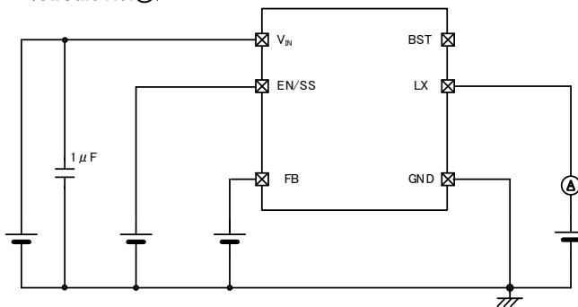
<Circuit No.⑦>
