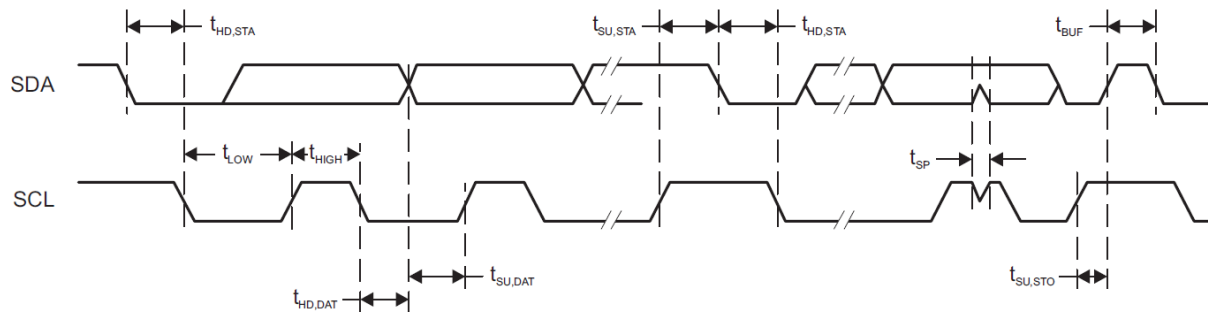
Figure 3.1 I²C Mode Timing
