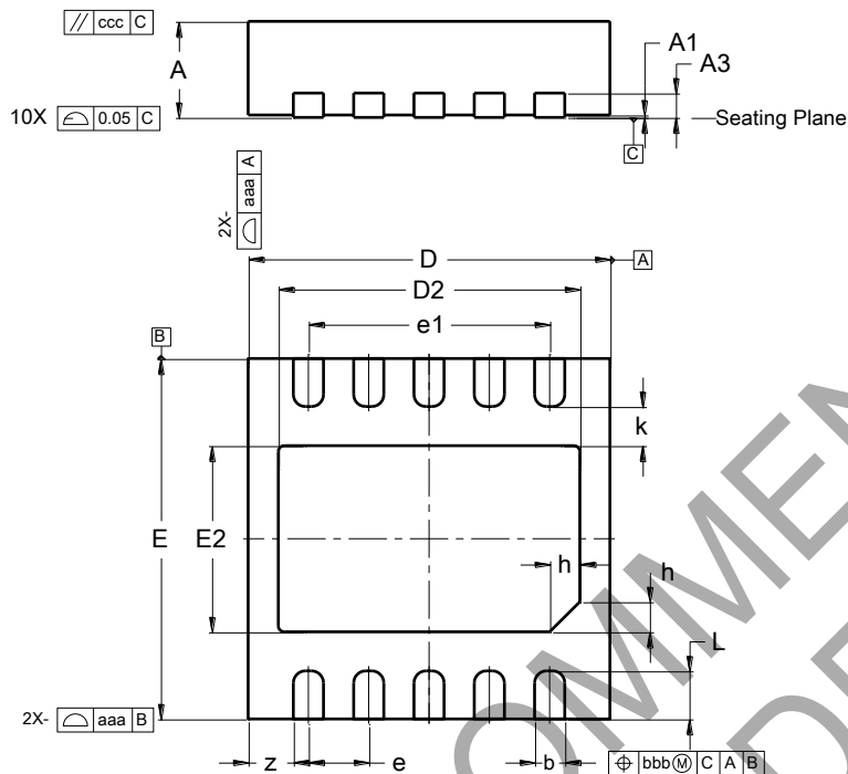
V-DFN3030-10 (Standard)
