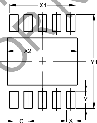
V-DFN3030-10 (Standard)
