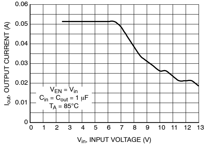
Figure 33. Measured Power Operating Area, 1.5 V, T_A = 85^\circ\text{C} , V_{\text{out\_drop}} = \text{max } 0.1 \text{ V}
