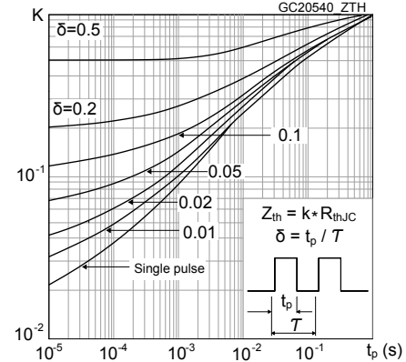
Figure 2. Thermal impedance
