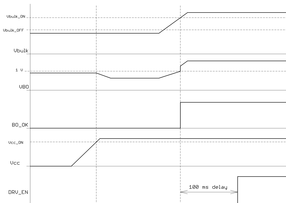
Figure 28. BO Input Functionality – V_{\text{bulk}} < V_{\text{bulk2}} , PFC Start Follows
