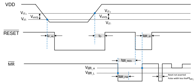
Figure 7-3. Timing Diagram \overline{MR} and \overline{RESET} (TPS3840DL)
