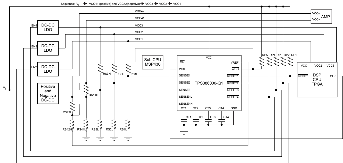
Figure 32. Application Schematic
