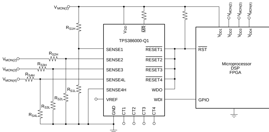
TPS386000-Q1 Typical Application Circuit
