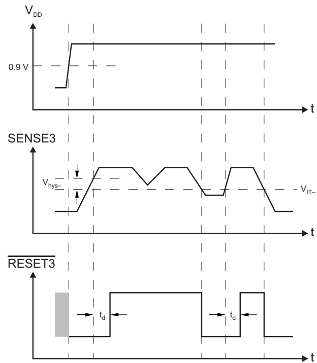
Figure 3. SVS-3 Timing Diagram
