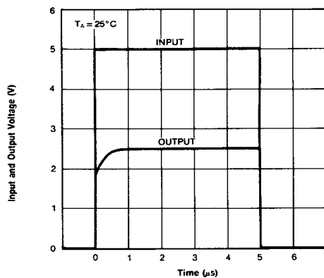
Figure 10. Pulse Response
