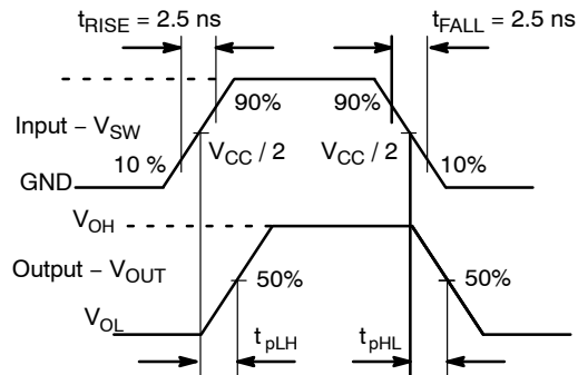
Figure 13. Propagation Delay
