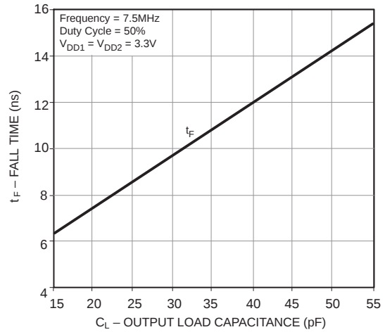
Figure 11. Typical Fall Time vs. Output Load Capacitance (Channel A &amp; B)
