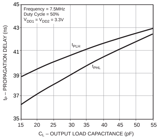
Figure 8. Typical Propagation Delay vs. Output Load Capacitance (Channel A &amp; B)
