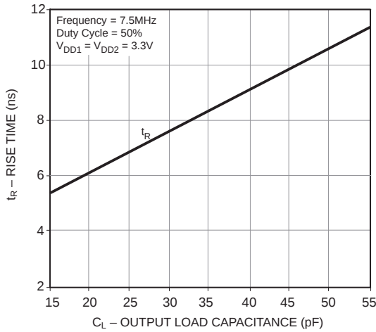
Figure 10. Typical Rise Time vs. Output Load Capacitance (Channel A &amp; B)
