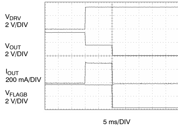
Figure 17. T_{\text{BLANK}} Response ( V_{\text{DRV}} signal forces the device to go into overcurrent conditions.)
