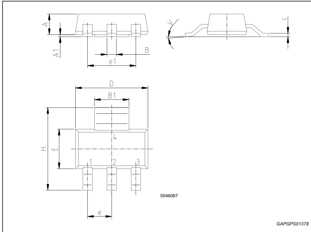
Figure 21. SOT-223 package outline
