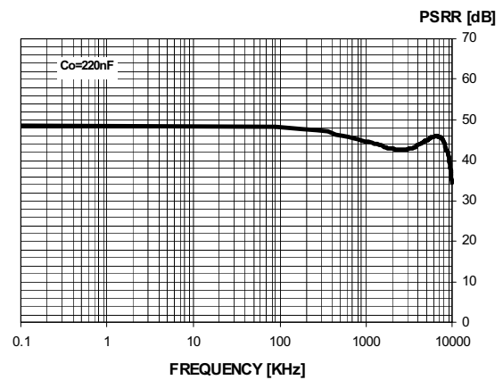
Figure 13. PSRR
