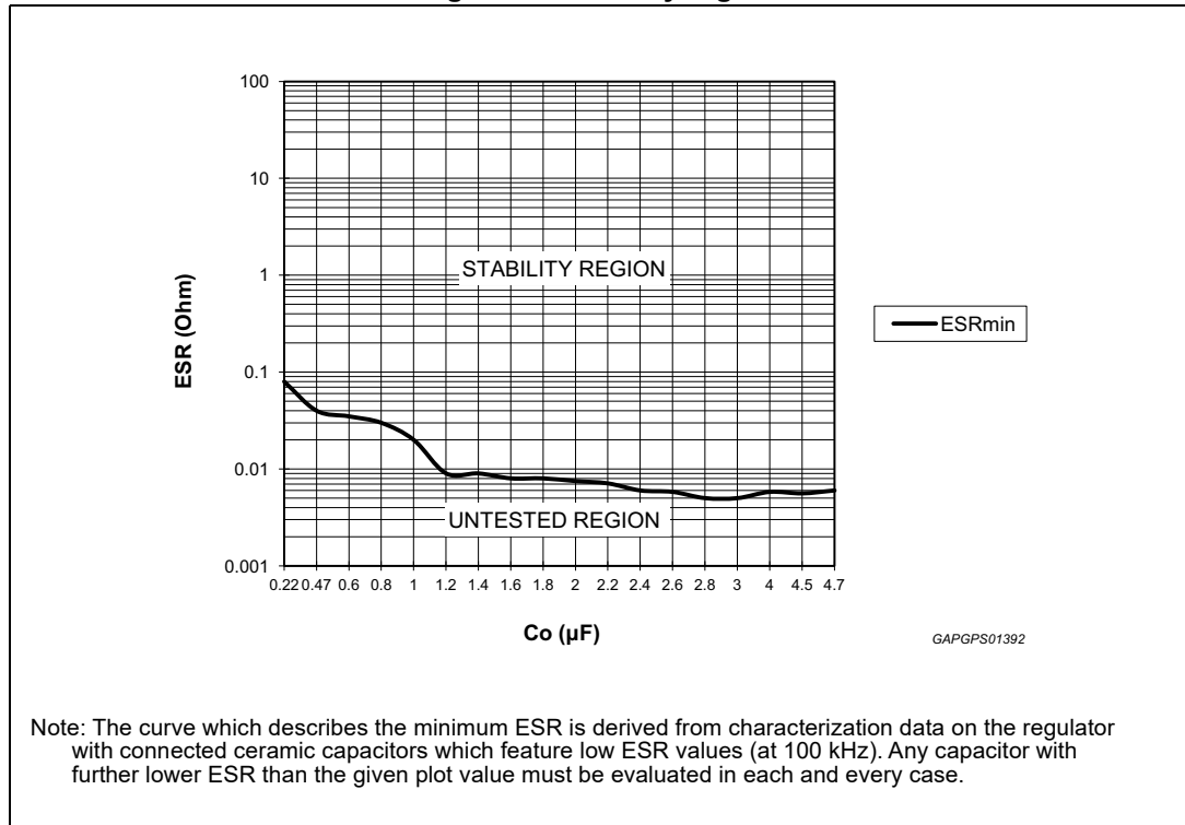
Figure 15. Stability region
