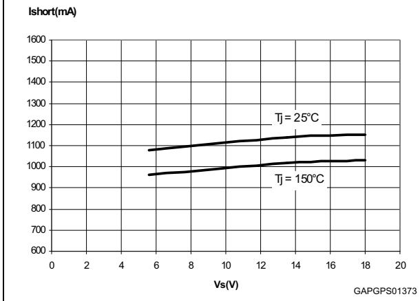
Figure 12. Short-circuit current vs. input voltage
