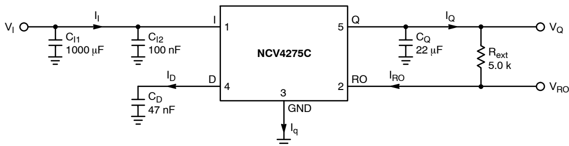
Figure 21. Test Circuit
