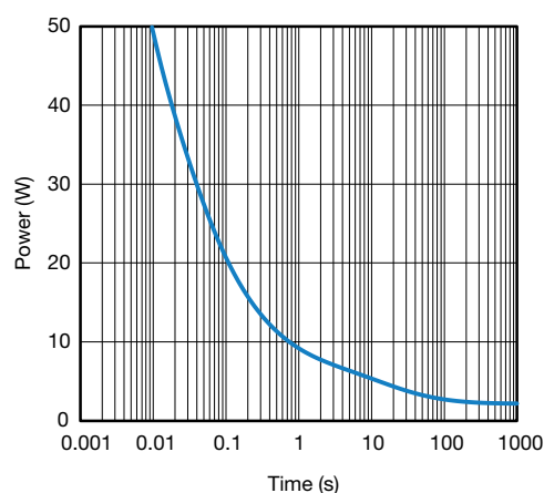
Single Pulse Power, Junction-to-Ambient
