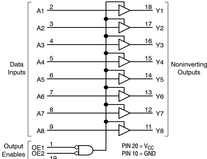
Figure 1. Logic Diagram
