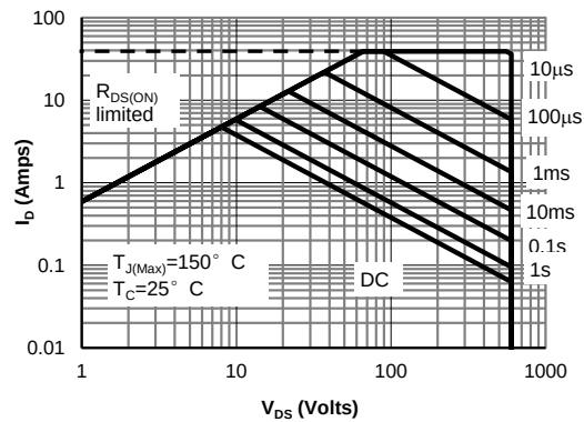
Figure 11: Maximum Forward Biased Safe Operating Area for AOTF11N60L (Note F)
