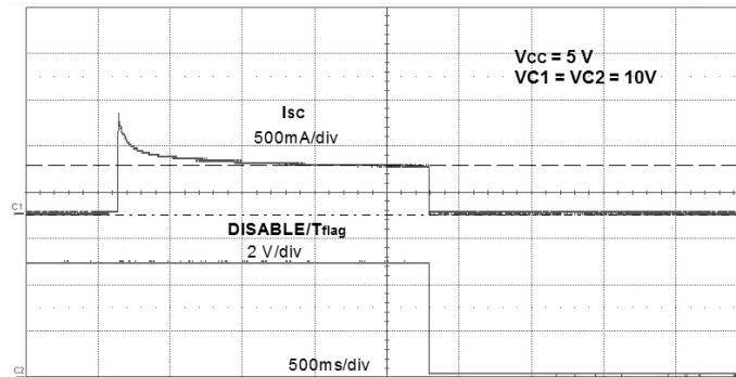
Figure 24. Output Short to Source. Output = V_{OL} Shorted to 12 V, T_A = 25\text{ }^{\circ}\text{C}
