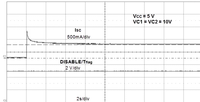
Figure 25. Output Short to Source. Output = V_{OL} Shorted to 12 V, T_A = -40\text{ }^{\circ}\text{C}
