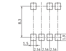
Recommended mounting pad ( TOP VIEW )
