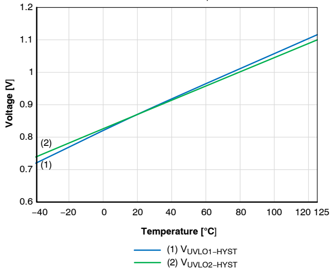
Figure 15. UVLO Hysteresis
